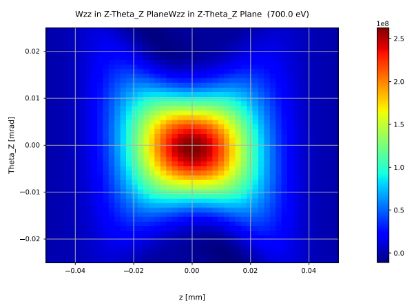
Fig. 16: Wigner distribution in source plane
