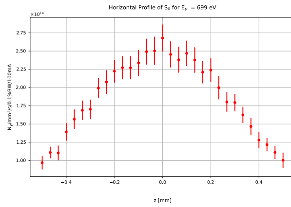
Fig. 11: Profile of flux-density in pinhole
