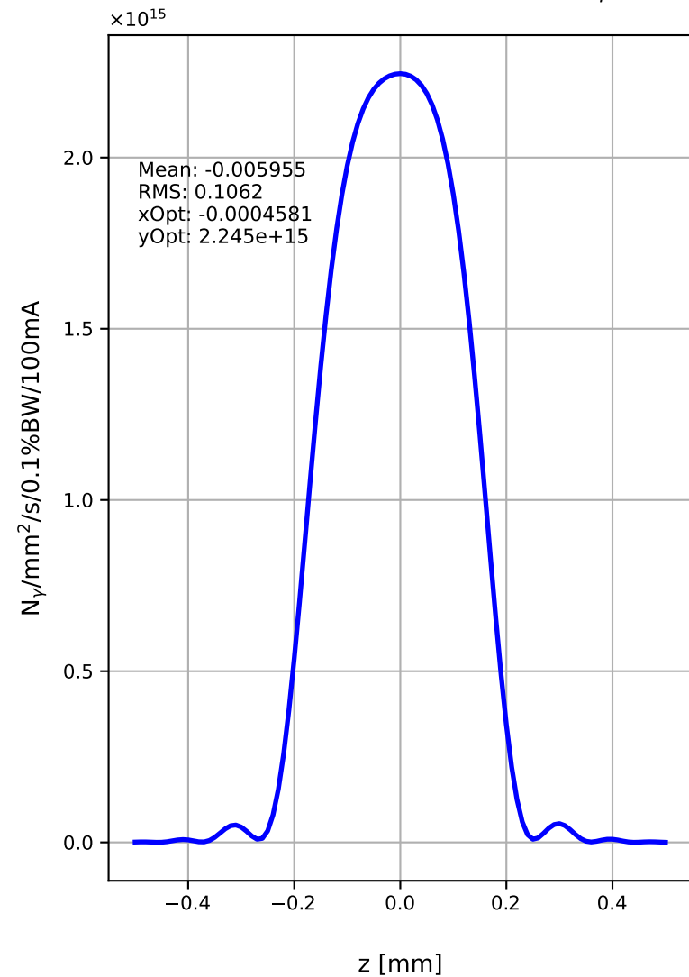
Horizontal Cut at x = 10.0\text{m} of S_0 for E_\gamma = 700\text{ eV}
