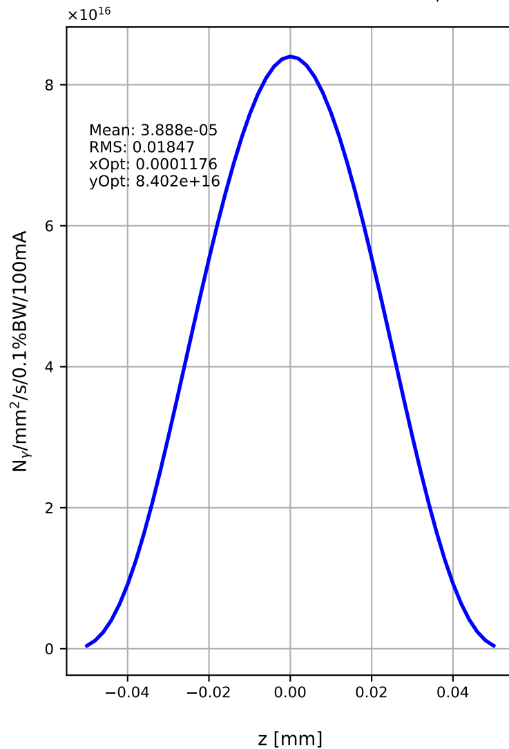
Horizontal Cut at x = 0.0\text{m} of S_0 for E_\gamma = 700\text{ eV}
