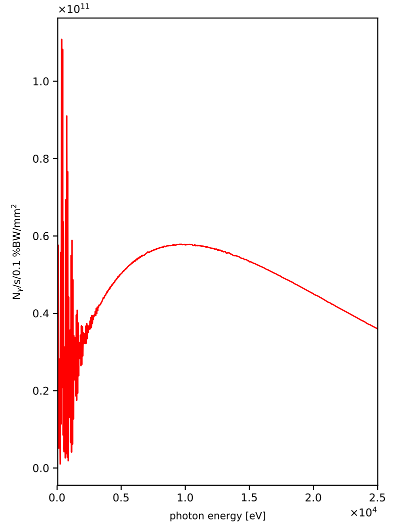
Density of S0 with e-spread at x=10.00 m, y=0.0 mm, z=0.0 mm
