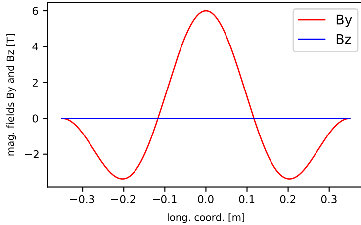
Magnetic field along trajectory
