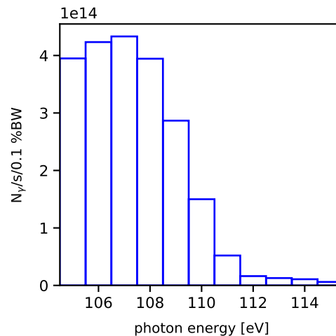
Flux with e-spread
