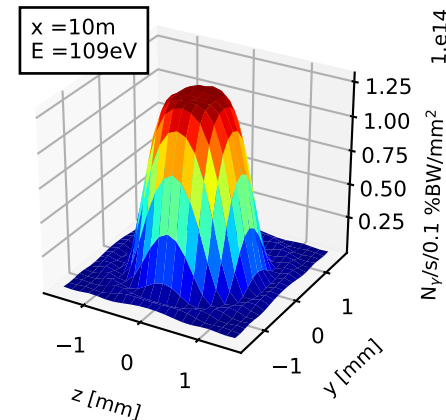
Density distribution of S0 with e-spread
