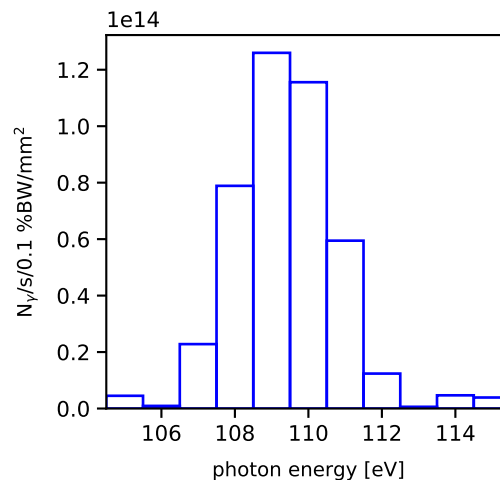
Density of S0 with e-spread at x=10.00\text{m} , y=0.0\text{mm} , z=0.0\text{mm}
