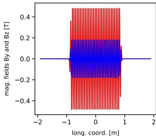
Magnetic field along trajectory
