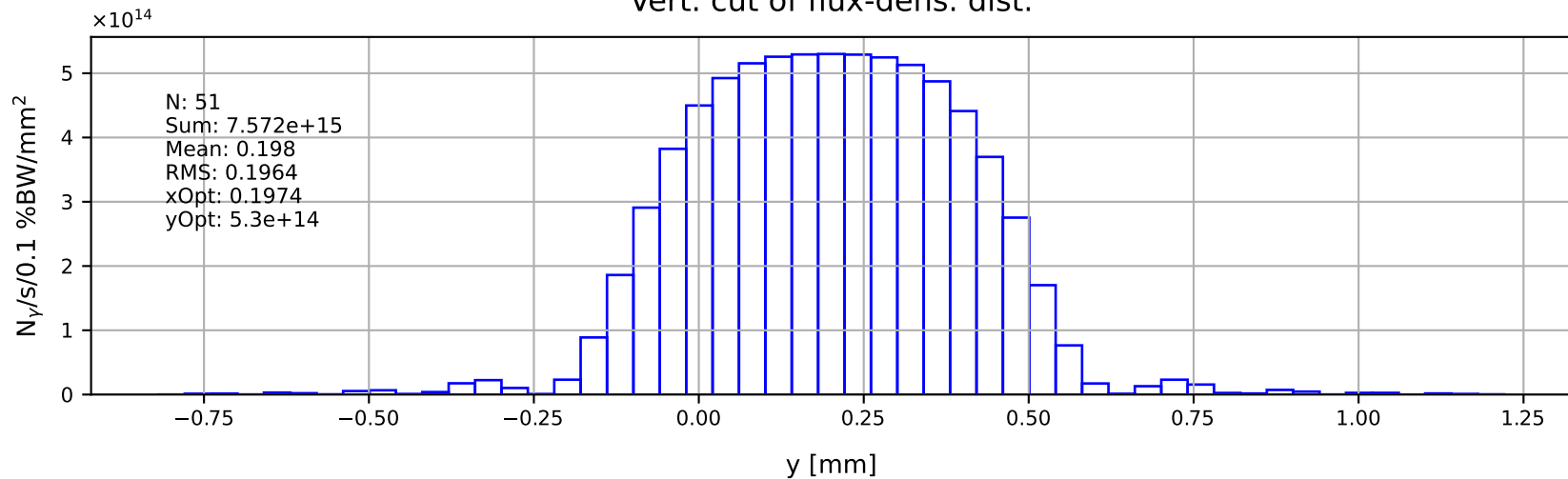
Vert. cut of flux-dens. dist.
