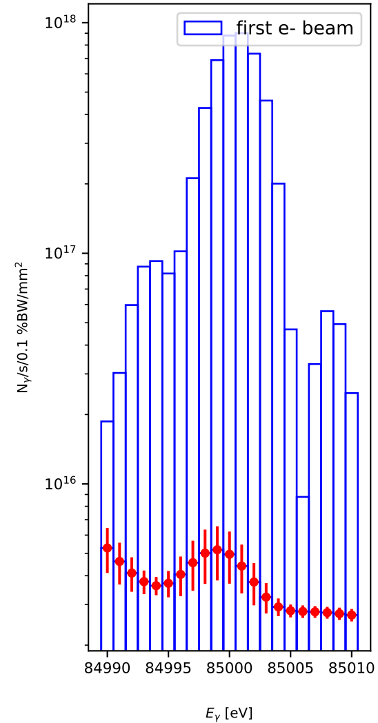
Single electron flux-density at x=250 m, y=0 mm, z=0 mm
