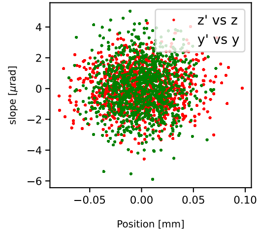
Phasespace at x=0 m
