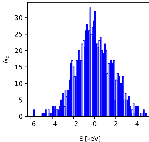
E-spread of 17.000 GeV beam at x=0 m
