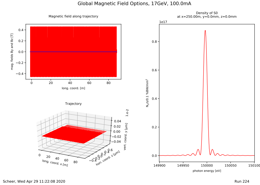
Fig. 26: Field and 9th harmonic of a long undulator section
