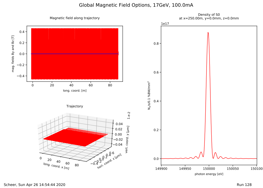
Fig. 28: Field and 9th harmonic of a long undulator section with continuous energy loss of the beam and corrected undulators
