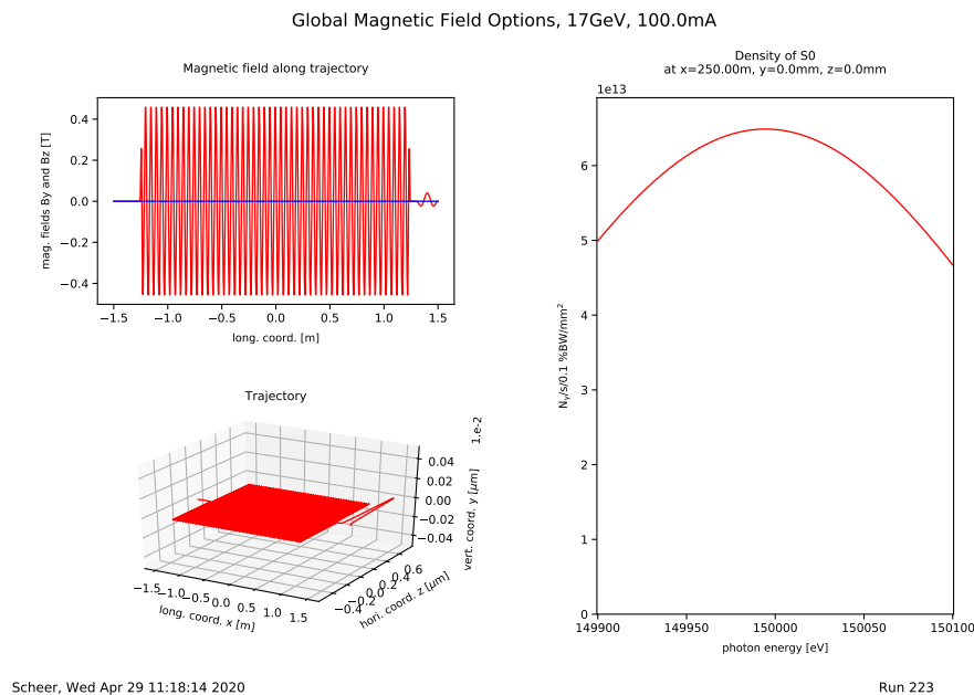
Fig. 25: Field and 9th harmonic of a single undulator section
