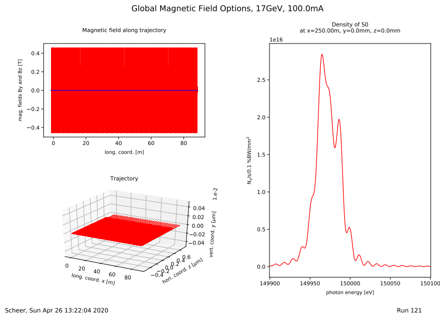
Fig. 27: Field and 9th harmonic of a long undulator section with continous energy loss of the beam
