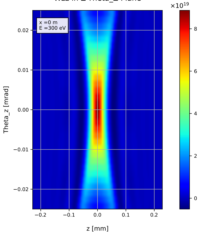
Wzz in Z-Theta_Z Plane
