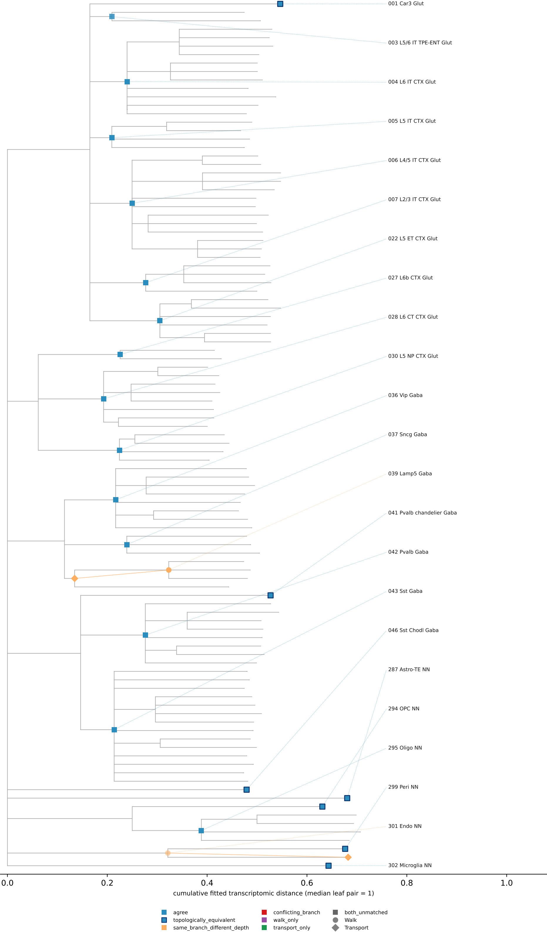
MetaArbor alignment phylogram (molecular; fit r=0.89, stress=0.10)
