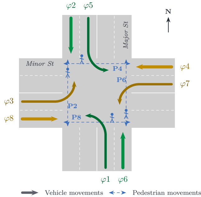
Figure 1: NEMA phase numbering as used by Load Std 8-Phase , per the FHWA convention. The main street runs north–south (green): southbound \phi_2 with its left \phi_5 , northbound \phi_6 with \phi_1 . The side street runs east–west (yellow): westbound \phi_4 with \phi_7 , eastbound \phi_8 with \phi_3 . Even = through, odd = protected left, and each left is numbered beside the opposing through. Pedestrian movements (dashed blue) carry the number of the through phase they walk with: P2/P6 cross the minor street alongside the main-street greens, P4/P8 cross the major street with the side-street greens.
