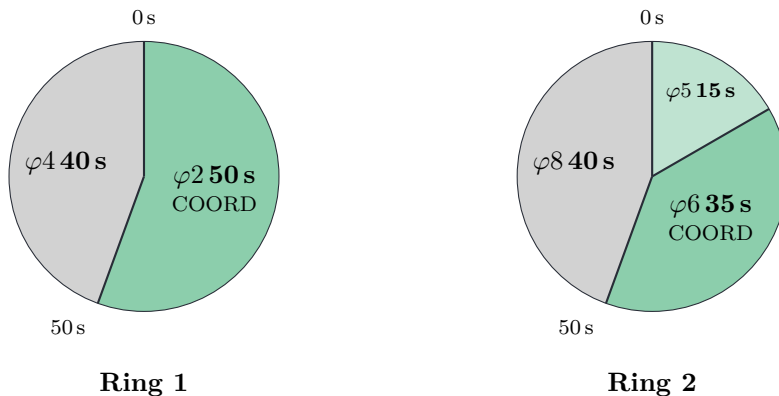
Figure 8: A 90-second cycle as two ring dials (phases 2/4 in ring 1; 5/6/8 in ring 2). The sweep position is the local cycle time, (\text{master clock} - \text{offset}) \bmod \text{cycle} . Both rings cross the barrier together at the 50s line.
