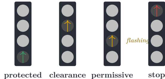
Figure 12: The four FYA states: green arrow during the protected phase, solid yellow during its clearance, flashing yellow while the opposing through is green, red otherwise. (Top three sections = the 3-section lens; bottom = the green-arrow add-on.)
