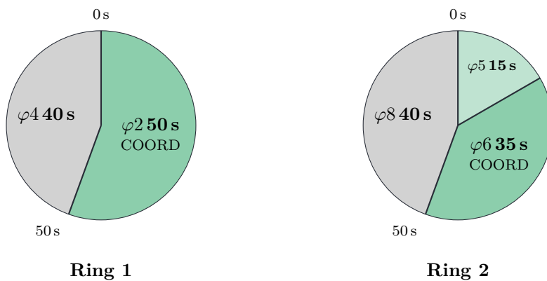
Figure 8: A 90-second cycle as two ring dials (phases 2/4 in ring 1; 5/6/8 in ring 2). The sweep position is the local cycle time , (master clock — offset) mod cycle. Both rings cross the barrier together at the 50s line.
