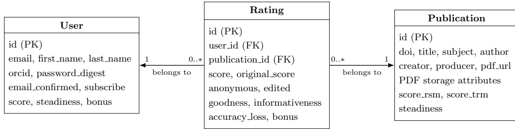
Figure 3: Persistent entities and associations in the RS_Server database (selected attributes).
