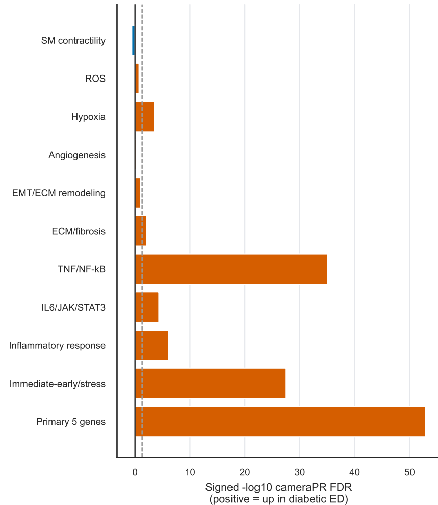
B. Ranked enrichment
