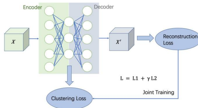
Ilustración 1 Diagrama de Deep Clustering Network (DCN) https://ieeexplore.ieee.org/stamp/stamp.jsp?tp=figure&arnumber=10047866
