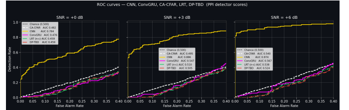
Fig. 2. Cell-level ROC curves at SNR=0, 3, and 6 dB (400 trials per panel, 5-bin oracle window). At SNR=0 dB: CNN 0.784, CA-CFAR 0.482, ConvGRU 0.476, LRT 0.459, DP-TBD 0.459. The CNN’s learned temporal features (max/mean/std across 10 sweeps) produce a 30-point AUC gain over the analytical integrators. LRT and DP-TBD match CA-CFAR despite accumulating all 10 sweeps, because moving-target energy is spread across cells, negating the stationary-target integration gain (see Section IV-B). ConvGRU’s modest cell-level AUC reflects that its hidden-state confidence is tuned for track confirmation, not raw discrimination; its operational advantage is in confirmed-track P_d (Table I).
