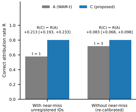
(b) Threat-model sensitivity
