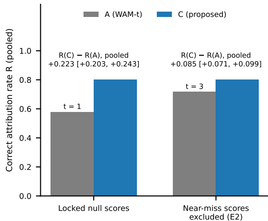
(b) Sensitivity to near-miss scores
