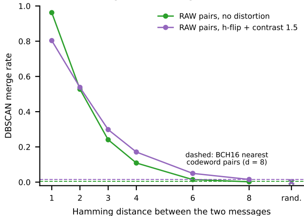
(a) Two messages in one image (test, 3,000)
