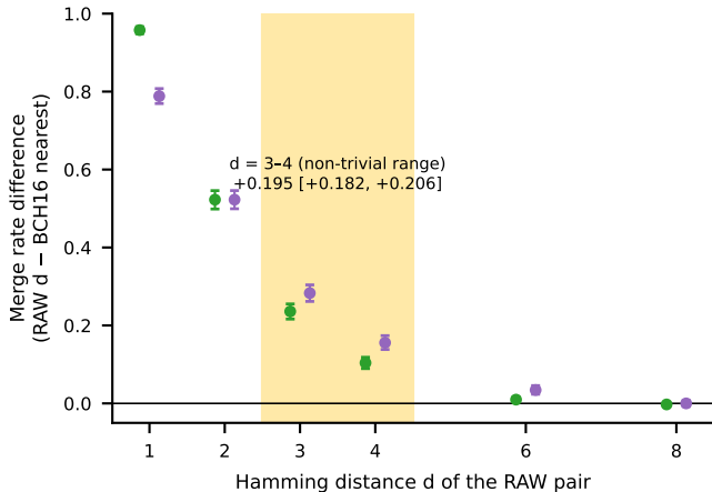
(b) Difference to distance-8 codewords (98.75% CI)
