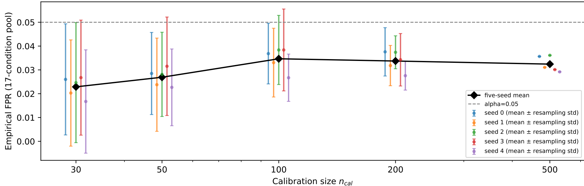
E4 calibration-size sensitivity (M3)
