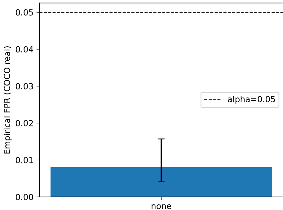
E7 COCO real-image FPR with Wilson 95% CI (M3)
