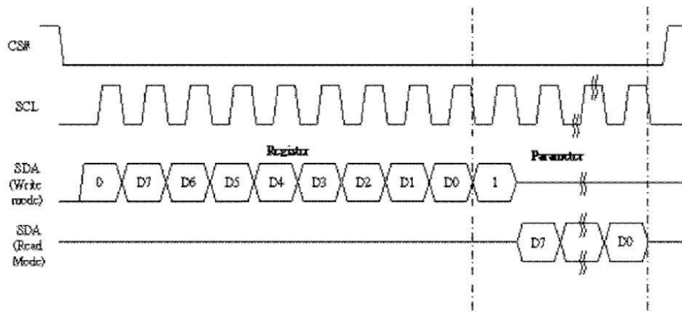
Figure 3.5-4: Read procedure in 3-wire SPI mode
