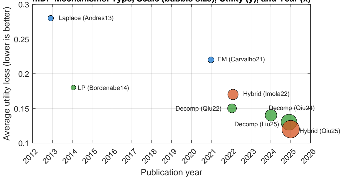
mDP Mechanisms: Type, Scale (bubble size), Utility (y), and Year (x)
