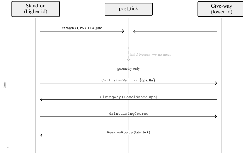
Figure 12: UML sequence for a successful CPA conversation ( MsgKind in comms.rs ). Failed P_{comms} draws omit all three messages and the waypoint. ResumeRoute is logged when the give-way ship finishes the avoidance queue (Table 8, step 5).
