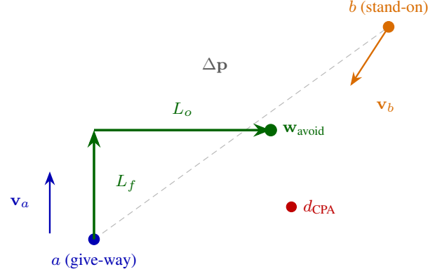
Figure 2: Give-way geometry. Ship a steers to a temporary waypoint \mathbf{w}_{\text{avoid}} placed L_f ahead and L_o to starboard (Eq. 6).
