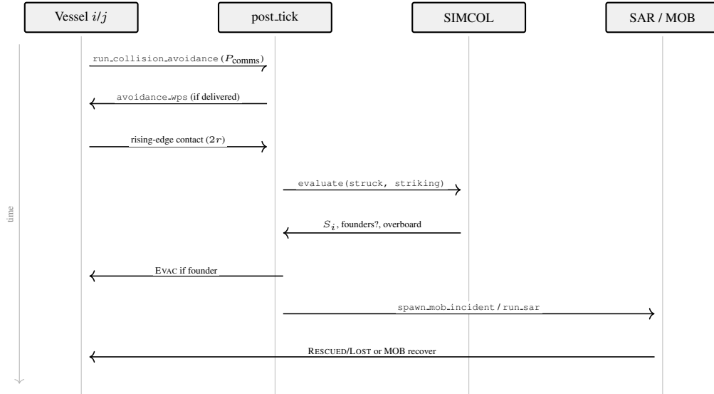
Figure 13: UML sequence aligned with post\_tick : CPA (or force-field) first, then hard contact, SIMCOL, run\_sar / run\_mob\_sar . Survival windows are liferaft ticks for EVAC and \tau_{mob} for persons in the water. Asset phases appear in Fig. 11.
