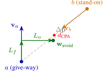
Figure 2: Give-way geometry. The lower-id vessel a turns to starboard toward a temporary waypoint w_{\text{avoid}} placed L_f ahead and L_o to starboard of its heading (Eq. 11), opening the closest-point-of-approach distance d_{\text{CPA}} to the stand-on vessel b . The manoeuvre executes only if the warning is delivered (Eq. 10).
