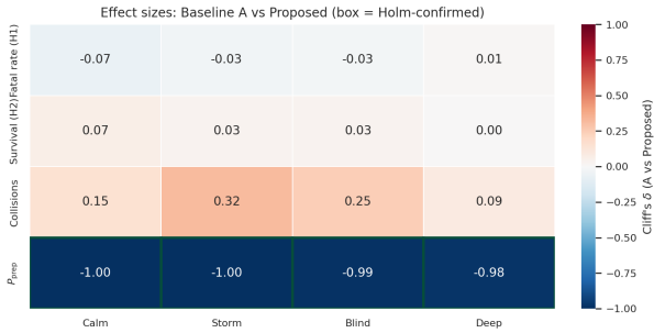
Figure 7: Cliff's \delta for Baseline A vs Proposed. Green boxes mark Holm-confirmed cells ( |\delta| \geq 0.2 , p_{\text{corr}} < 0.05 ).
