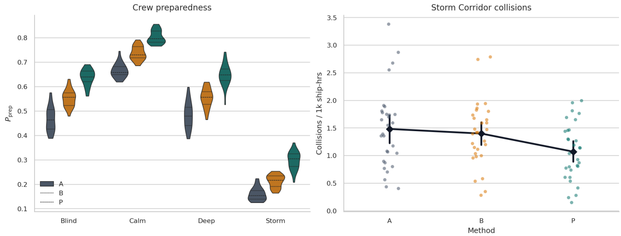
Figure 8: Left: P_{prep} violins (definitive). Right: Storm Corridor collision strip with mean \pm 95\% CI.
