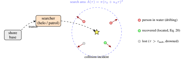
Figure 4: Man-overboard search. A collision spawns one incident whose casualties (Eq. 15) become individual persons-in-water, each scattered about the impact point and advected along its own drift bearing (red arrows). A single searcher — chosen by the same nearest-base, helicopter-versus-patrol rule as the liferaft chain — transits from a shore base and homes on the cluster centroid, then draws the Koopman detection (Eq. 20) independently per person over the drift-growing search area, so individuals are recovered (green) as they are located. Anyone not reached before the cold-water survival window \tau_{\text{mob}} elapses is lost (grey). Unlike the whole-group liferaft case of Fig. 3, each casualty resolves separately.
