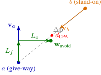
Figure 2: Give-way geometry. The lower-id vessel a turns to starboard toward a temporary waypoint \mathbf{w}_{\text{avoid}} placed L_f ahead and L_o to starboard of its heading (Eq. 11), opening the closest-point-of-approach distance d_{\text{CPA}} to the stand-on vessel b . The manoeuvre executes only if the warning is delivered (Eq. 10).
