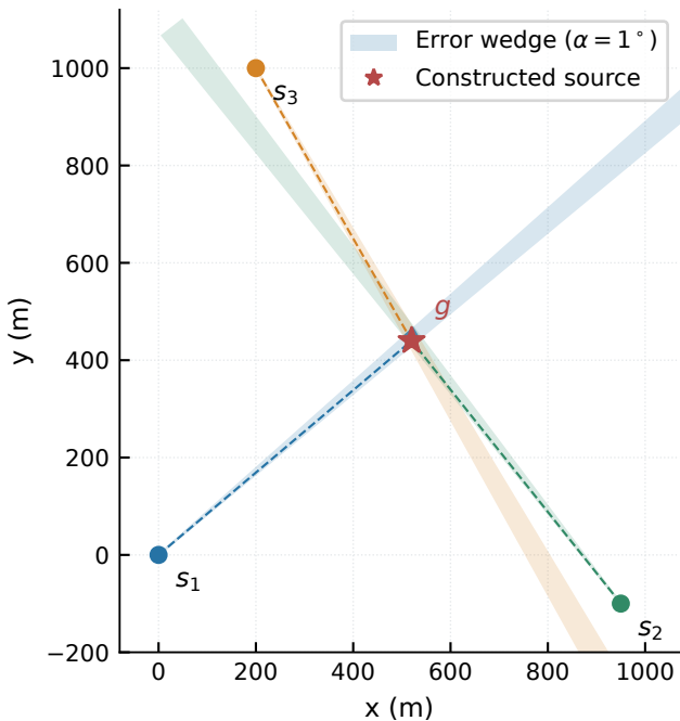
(a) Three bearing observations
