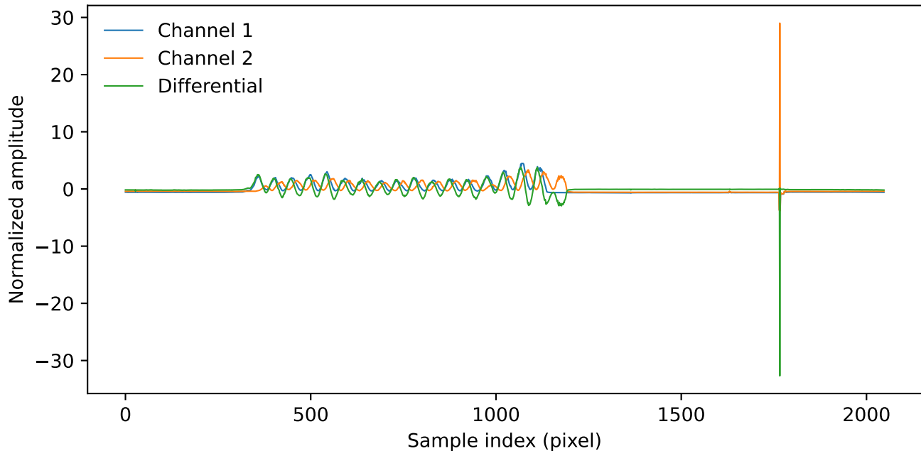
Representative waveform, 199.2 mm
