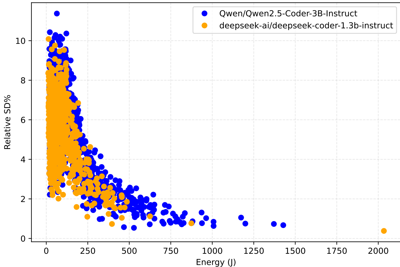
Relative Energy deviation within task
