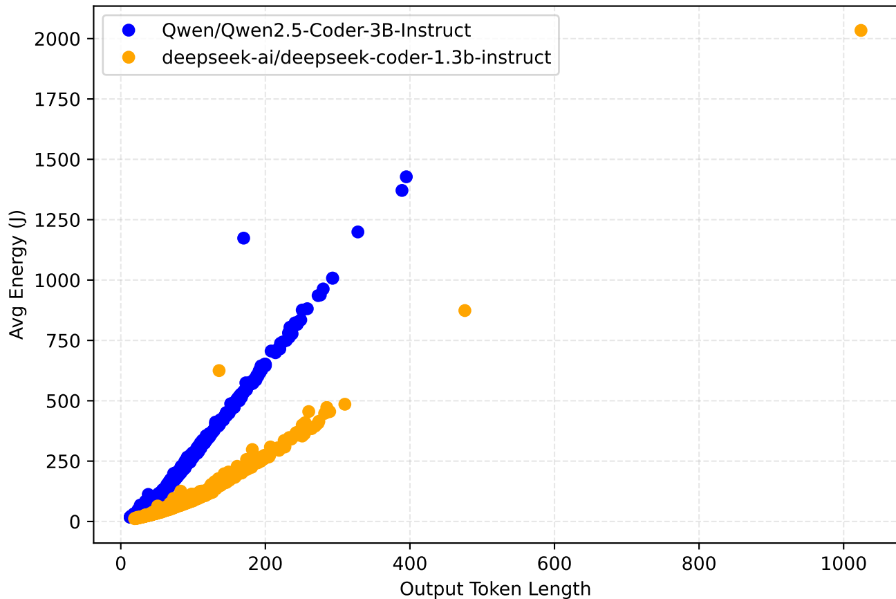
Energy vs Output Token Length by Model
