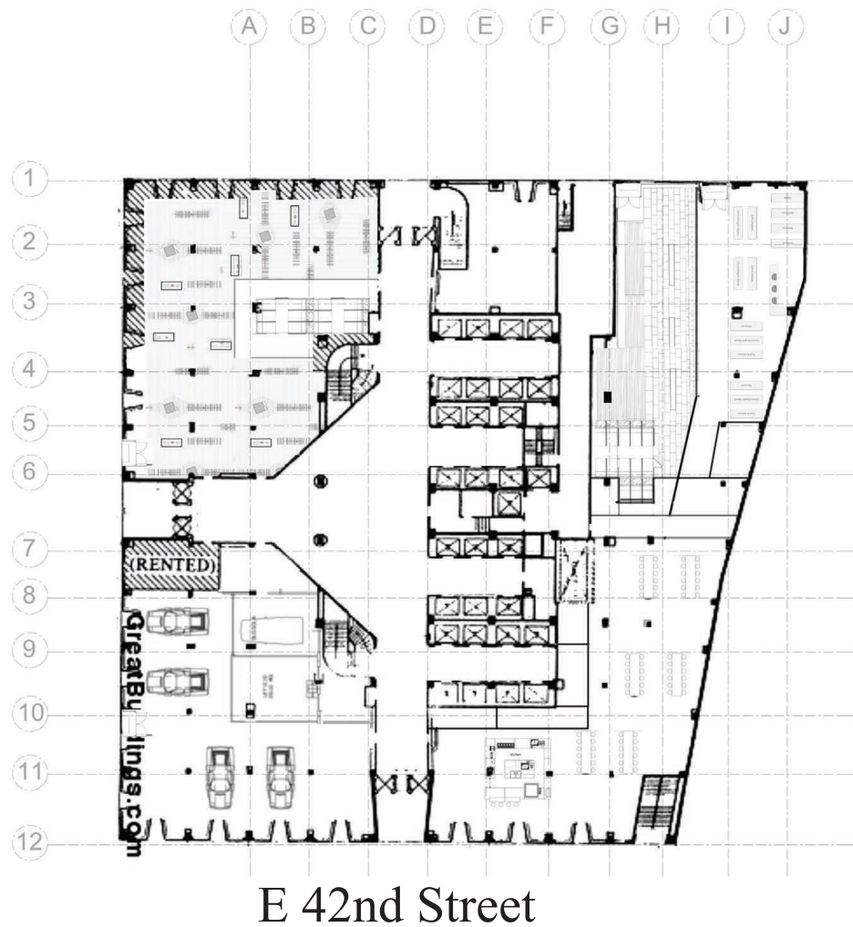
(Figure 8-GF Plan)
