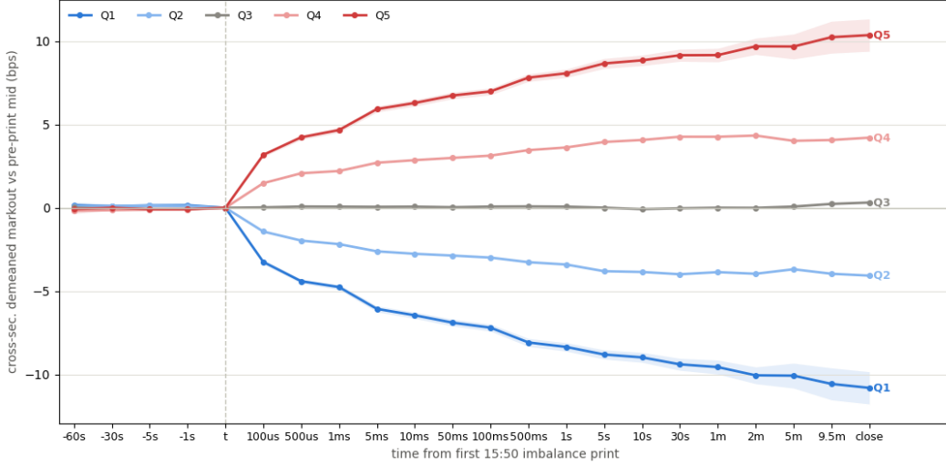
Figure 3: Returns Markout over Forecast Horizon Bucketed by Feature Quintiles
