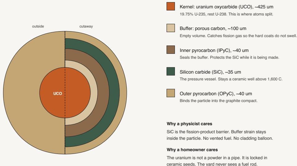
Figure 9. One TRISO particle (typical of the class, not a shop drawing)
