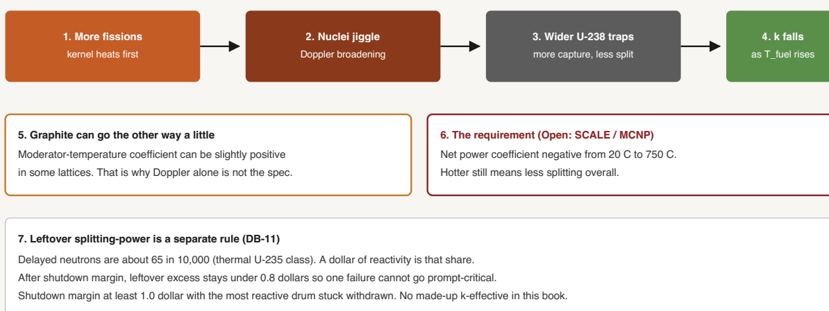
Figure 26. From hotter fuel to the Doppler requirement
