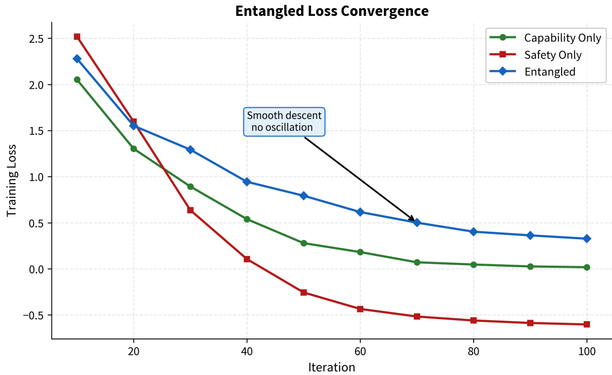
Figure 2. Training loss convergence for all three conditions over 100 iterations. The entangled loss (blue diamonds in the raster) descends smoothly without oscillation, indicating that safety and capability gradients cooperate rather than conflict. Colour key in the raster legend: green circles = capability_only; red squares = safety_only; blue diamonds = entangled.
