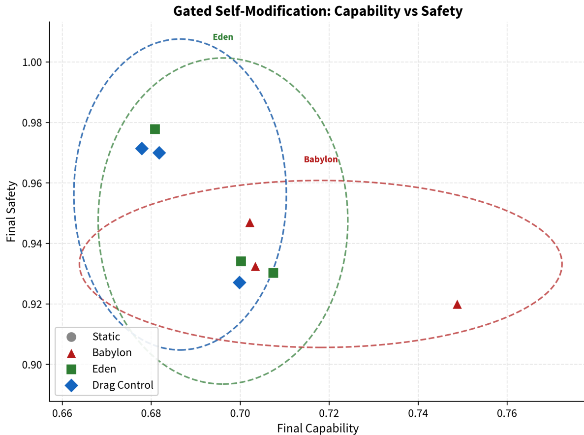
Figure 4. Capability vs safety for all 12 gated simulation runs (4 conditions, 3 seeds each). Babylon (red triangles) drifts toward higher capability at the expense of safety. Eden (green squares) maintains balanced performance. Static (grey circles in the legend) and Drag Control (blue diamonds) produced identical mean values (both at capability 0.687, safety 0.956; see §5.2 table), so the Static markers sit beneath the Drag Control markers in the raster and are hidden by them; this exact overlap is the verification-tax finding: the tax comes from checking, not from safety.
