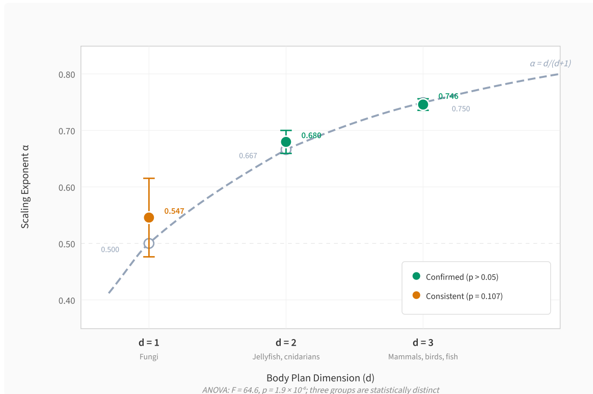
Figure 9 | The Dimensional Ladder. Dashed curve: the \alpha = d/(d+1) prediction (independently derived by West et al. 1997, Banavar et al. 2010, Demetrius 2010, Zhao 2022, Bettencourt 2013). Open circles: predicted values. Filled circles: published measurements with \pm 1\sigma error bars. Green: confirmed. Amber: consistent but requiring individual-hypha respirometry. The dimensional generality of the formula predicts how fungi, jellyfish, and mammals all metabolise energy; three correct predictions across three domains of life. Note: the paper's later analysis (see §3.6 and §3.7) records that 2D biology is under review pending identification of a valid 2D biological test organism; the jellyfish datum shown here reflects the earlier tabulated result (mean 0.680) and is retained as evidence pending reconciliation of the 2D biology entry across sections.
