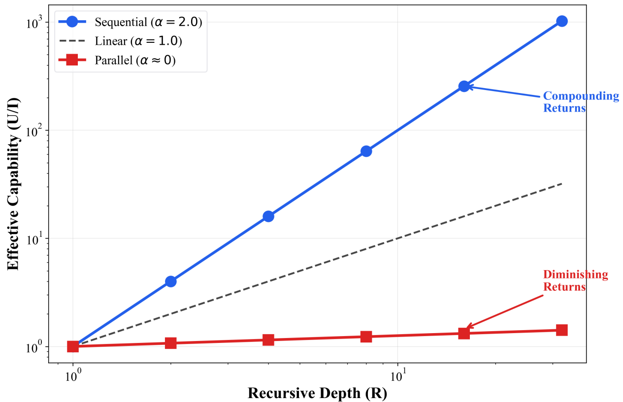
Figure 3 | Scaling Comparison. Log-log plot showing different scaling regimes. Power law U = R^\alpha appears as a straight line with slope \alpha . Sequential recursion ( \alpha > 1 ) illustrates super-linear growth schematically; parallel sampling ( \alpha < 1 ) shows diminishing returns. The ARC Principle originally predicted \alpha_{\text{sequential}} > 1 > \alpha_{\text{parallel}} ; Paper II's multi-model replication (March 2026, see §3.9) confirms \alpha_{\text{parallel}} \approx 0 universally, while the best cross-architecture fit for \alpha_{\text{sequential}} is sub-linear ( \approx 0.49 , Gemini 3 Flash). The directional prediction (sequential > parallel) holds robustly across all six frontier models; the quantitative \alpha > 1 claim is not confirmed cross-architecturally for current frontier systems.
