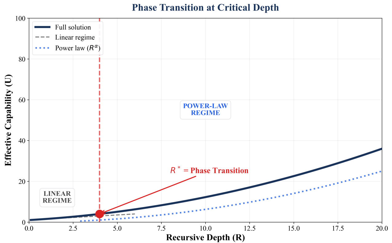
Figure 14 | The Scaling Crossover at R^* . Below the critical depth R^* , base capability ( I ) dominates and scaling appears linear. Above R^* , recursive compounding dominates and scaling becomes power-law. This crossover point is the depth at which recursive amplification becomes dominant. Systems should exhibit a distinct "elbow" in their capability curves at R^* .
