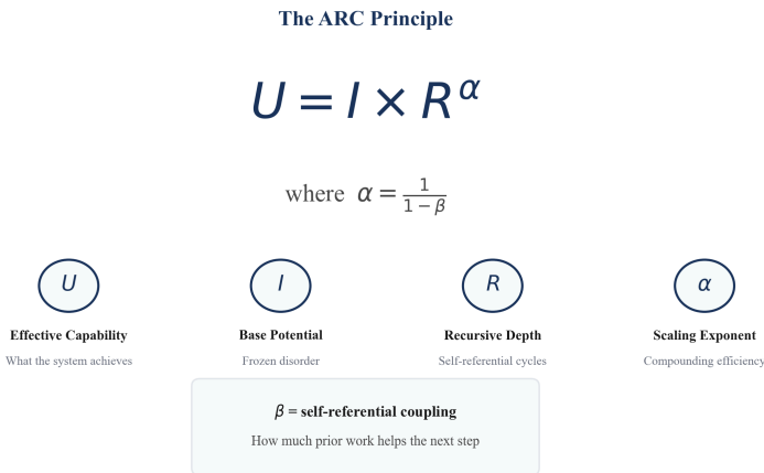
Figure 1 | The ARC Equation. Effective capability (U) equals base potential (I) multiplied by the amplification factor g(R). For recursive intelligence, \alpha = 1/(1-\beta) where \beta measures self-referential coupling. For physical systems, \alpha = d/(d+1) where d is the network dimension (always < 1 ); this form was independently derived by West et al. (1997), Banavar et al. (2010), Demetrius (2010), Zhao (2022), and Bettencourt (2013). The ARC Bound ( \beta \leq 0.5 , \alpha \leq 2 ) defines the maximum safe scaling for recursive intelligence.
