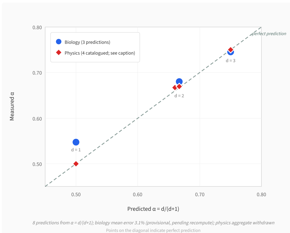
Figure 10 | Predicted vs Measured. Eight cross-domain predictions from one formula: \alpha = d/(d+1) . Blue circles: biological systems (fungi at d=1 , jellyfish at d=2 , mammals at d=3 ). Note: the d=2 datum (jellyfish, measured \alpha = 0.680 ) is under review in the paper's later analysis (§3.6, §3.7); it is retained here as plotted evidence pending reconciliation of the 2D biology entry across sections. Red diamonds: physics systems (crystal growth, phase transitions, fracture; earthquake data point removed; retained separately as a variable-pair case study). Every remaining point falls on or near the diagonal of perfect prediction. A single equation, with zero adjustable parameters, governs systems spanning biology, geophysics, and condensed matter physics.
