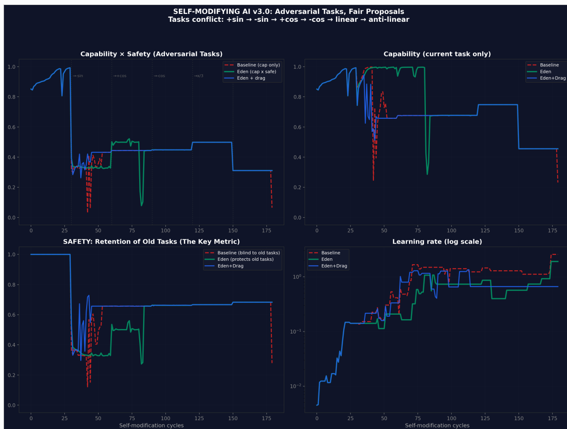
Figure 3. Adversarial self-modification in PaperVI's v3 run: no condition separated on collapse. v3 adversarial self-modification (20 seeds, 180 cycles, deliberately conflicting tasks: +\sin , -\sin , +\cos , -\cos ). Eden + Drag and the capability-only baseline both recorded zero collapses; the run's only collapse was a plain-Eden seed (Fisher p = 1.0 ). What the run separated was safety retention, ordered baseline 0.602, Eden 0.650, Eden + Drag 0.681 (Mann-Whitney p = 0.0015 ). Placed here because Paper III's alignment-scaling half reports depth contrasts compatible with the problem (external safety not co-scaling with capability) and PaperVI tests one direction for the fix: capability-safety entanglement. In these toy networks the entangled conditions retained more safety than the baseline; on collapse they did not differ from it.
