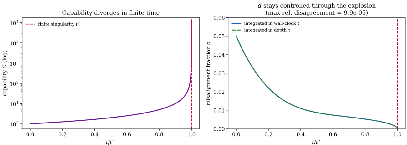
Figure 7. A hard takeoff is regular in the depth clock (Depth-Regularity Theorem, Theorem 3). [Internal verification of Eq. (1), not real-system data] Left: capability diverges to \sim 10^5 at a finite singularity time t^* . Right: the misalignment fraction is driven to zero as the explosion is approached. Integrating in wall-clock time and in self-improvement depth \tau give identical trajectories (max disagreement 9.9 \times 10^{-5} ). Placed here because it is the technical basis for the "non-linear time makes coordinate properties look absolute" move of $6.3 and $11.9A (Signature S5, time crystals): a property that
