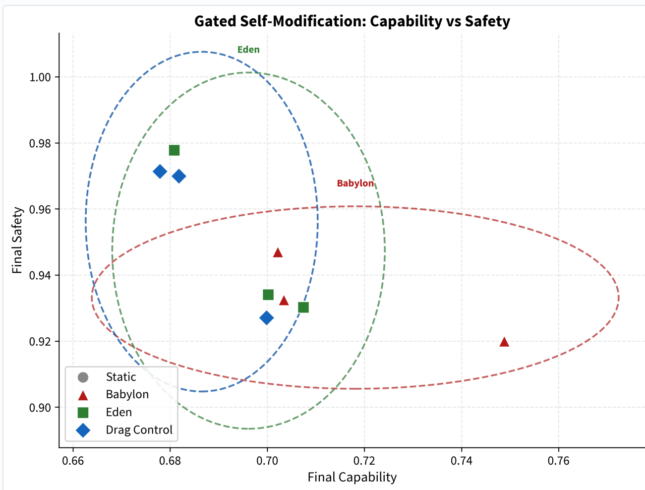
Figure 2. What phase 1 actually buys, at 12 seeds. Capability vs safety for 12 gated self-modification runs (4 conditions, 3 seeds each). Babylon (red, unconstrained) drifts toward higher capability at the expense of safety. Eden (green, gated) maintains balanced performance. Static and Drag Control cluster identically, confirming the "verification tax" comes from checking, not from safety. Placed here because the plot is the visual form of the phase-1 delay-buying claim of this section: gated self-modification preserves safety at a modest speed cost while unconstrained self-modification trades safety for speed.
