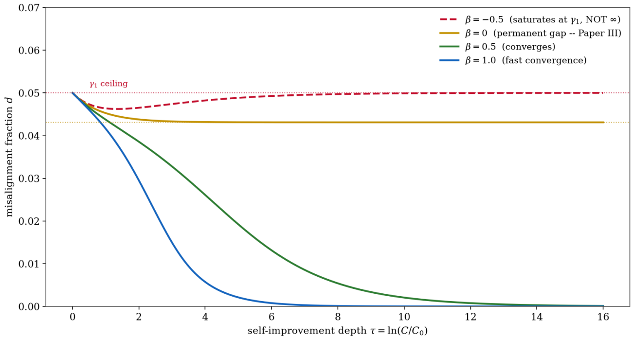
Figure 6. The \beta > k criterion in one plot. [Internal verification of Eq. (1), not real-system data] \beta > 0 drives the misalignment fraction d to zero; \beta = 0 holds a permanent gap; \beta = -0.5 saturates at the drift coefficient \gamma_1 (bounded, not divergent). Placed here because it is the direct visualisation of the load-bearing quantity that Paper X moved the safety criterion to. The dotted ceiling at \gamma_1 is never breached (correction of an earlier draft's divergence claim recorded in Theorem 2).
