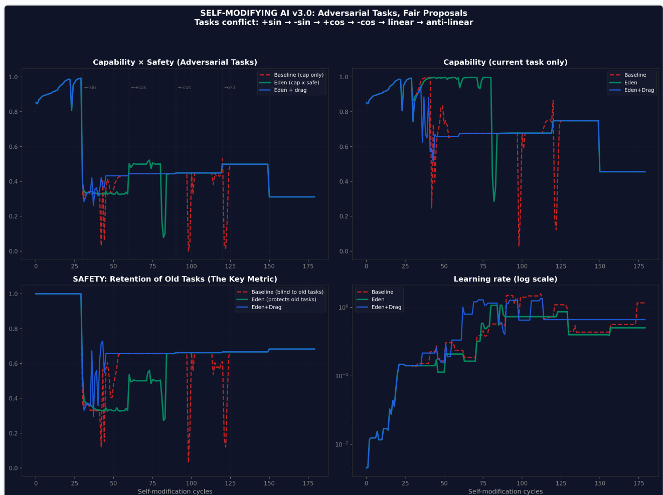
Figure 3. Entangled architectures hold; externally-constrained systems collapse. v3 adversarial self-modification (20 seeds, 180 cycles, deliberately conflicting tasks: +\sin, -\sin, +\cos, -\cos ). Baseline collapses; Eden Entangled and Eden + Drag hold, with Eden + Drag achieving zero collapses across all 20 seeds. Placed here because Paper III's alignment-scaling half locates the problem (external safety does not co-scale with capability) and Paper VI shows the direction in which the fix lies: capability-safety entanglement rather than external constraint. Together the two provide the live-system evidence base for the correction requirement.
