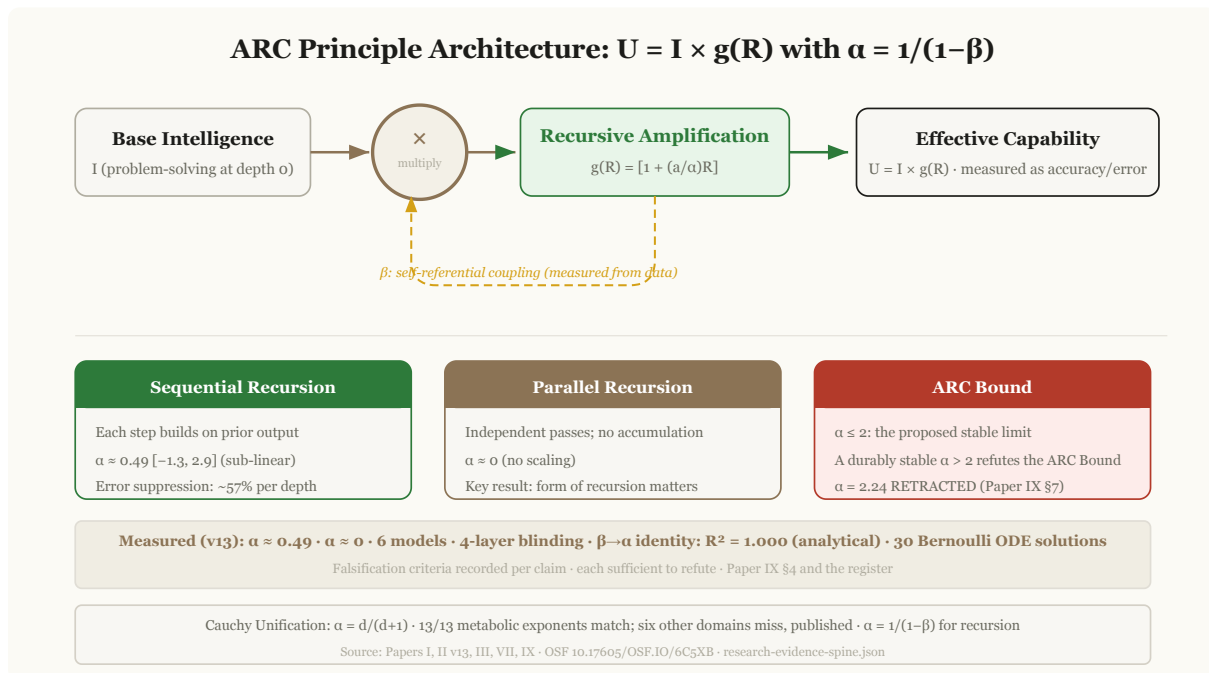
Figure 1 | ARC Architecture and Cauchy Unification. Four functional equations (Cauchy 1821) constrain scaling to four families: linear, power law, exponential and logarithmic. \alpha = d/(d+1) for physical systems (13/13 nearest-comparator matches at the taxon grain, reported by tier and never blended; the largest modern mammalian dataset gives 0.687, 95% CI 0.674 to 0.701, which excludes 0.750, see §7.1); \alpha = 1/(1-\beta_L) for recursive intelligence (the self-reference theorem; in the artwork \beta is drawn bare, carrying no subscript), one of the two routes to the value two; the second is the ARC Ceiling \alpha_{\text{crit}} = 1/(1-\gamma) , and whether the pair agree away from \beta_L = \gamma = 0.5 is a drafted test, preregistered by timestamp and awaiting human submission. 19/25 domains confirm predicted function family ( p = 7 \times 10^{-5} , permutation; six-model set, no logarithmic candidate - §3.2). The rerun of 11 August 2026, which added the logarithmic candidate, returns 18/25. Source: Paper VII · Foundational · evidence spine C-4, C-11.
