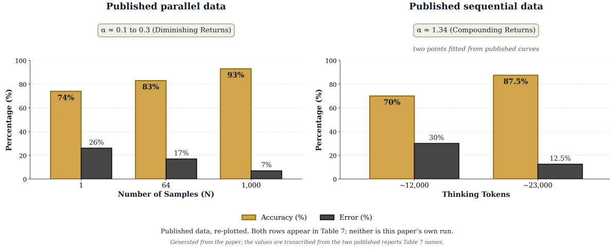
Figure 3 | Published data, re-plotted. Left: the parallel series of a published report on AIME 2024, \alpha \approx 0.1 - 0.3 ; its three points are a single sample, consensus among 64 samples at 83% and a re-ranking of 1,000 samples with a learned scoring function at 93%, so the range spans two methods and not one. Right: the sequential curves of a published report on AIME 2025, two points fitted in Paper I, \alpha \approx 1.34 ; the two points are two versions of one model, each at its own average token use, and not two thinking budgets of a single version. The panels are two exams and two models. Both rows appear in Table 7; neither is this paper's own run.
