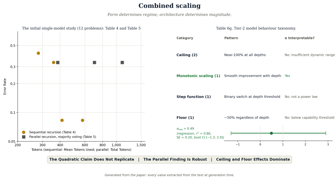
Figure 15 | Combined scaling: the initial single-model study (DeepSeek, 12 problems) + the six-model study (5 models, 30 problems). Sequential \alpha > 0 for every measurable model; parallel \alpha \approx 0 universally. Magnitude architecture-dependent. Form determines regime; architecture determines magnitude.
