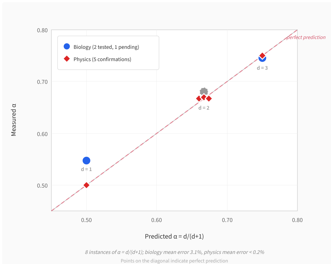
Figure 2 | Predicted vs Measured. Cross-domain instances of one independently derived formula: \alpha = d/(d+1) [17,21,22,23,24,25]. Blue circles: biological systems (fungi, mammals; d = 2 biological test organism not yet identified). Red diamonds: physics systems (crystal growth, phase transitions, fracture, earthquakes). Points on or near the diagonal indicate accurate prediction. A single equation, with zero adjustable parameters, governs systems spanning biology, geophysics, and condensed matter physics. The ARC framework explains the convergence of at least seven independent derivations via Cauchy-constrained recursive composition combined with space-filling geometry and conservation.
