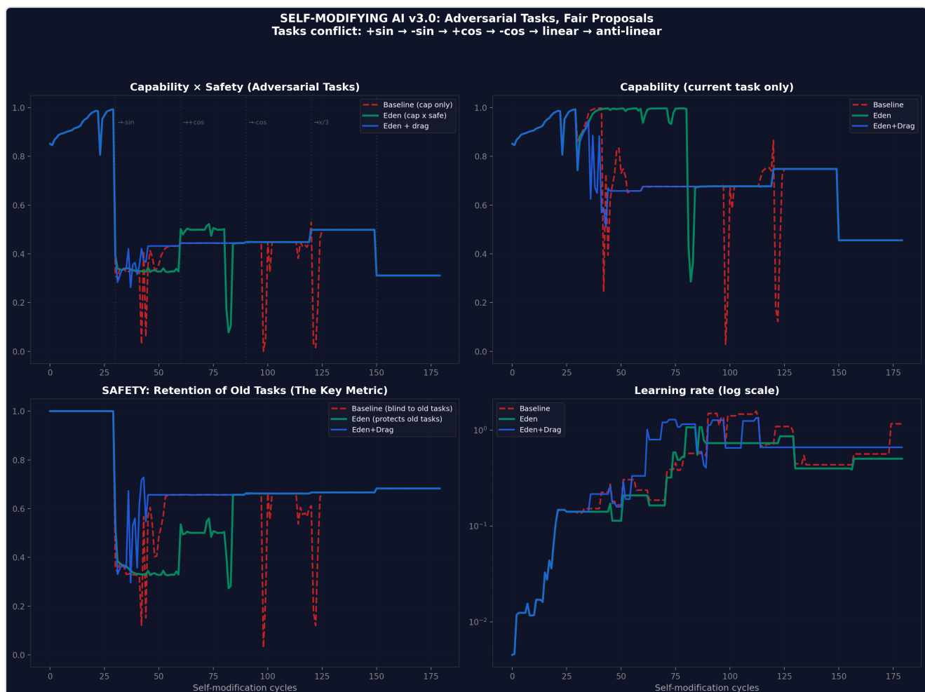
Figure 3. Entangled architectures hold; externally-constrained systems collapse. v3 adversarial self-modification (20 seeds, 180 cycles, deliberately conflicting tasks: \rightarrow \sin , \rightarrow -\sin , \rightarrow +\cos , \rightarrow -\cos ). Baseline collapses; Eden Entangled and Eden + Drag hold, with Eden + Drag achieving zero collapses across all 20 seeds. Placed here because Paper III's alignment-scaling half
