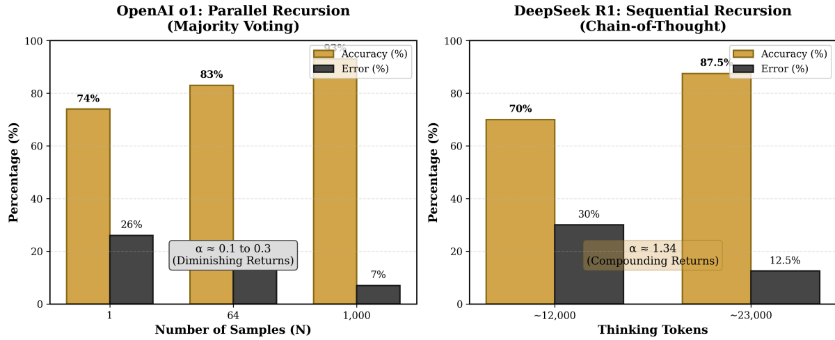
Figure 3 | Published data, re-plotted. Left: parallel sampling with majority voting, \alpha \approx 0.1 - 0.3 . Right: the sequential curves of a published report, two points fitted in Paper I, \alpha \approx 1.34 . Both rows appear in Table 7; neither is this paper’s own run.
