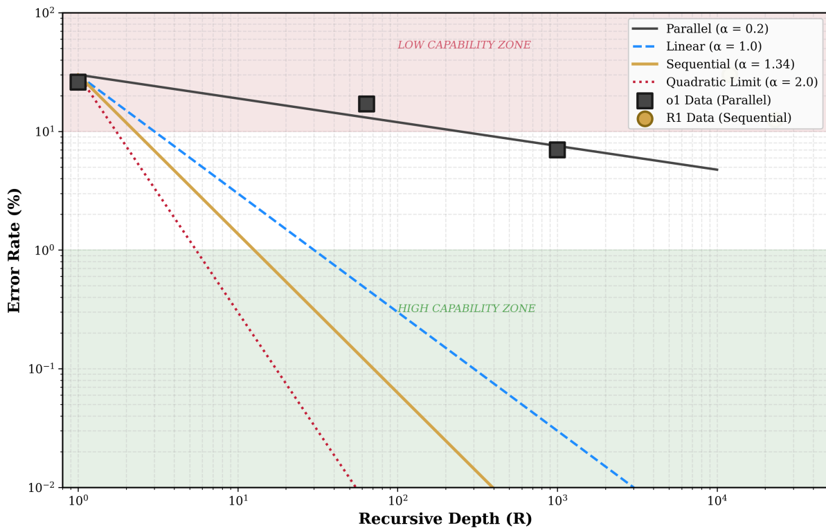
Figure 4 | Log-log comparison: sequential (gold) shows positive scaling; parallel (grey) flat. The series plotted are the two published sources of Table 7; the cross-architecture result is at Figures 7 and 10. Power law U = R^{-\alpha} as straight line on log-log axes.
