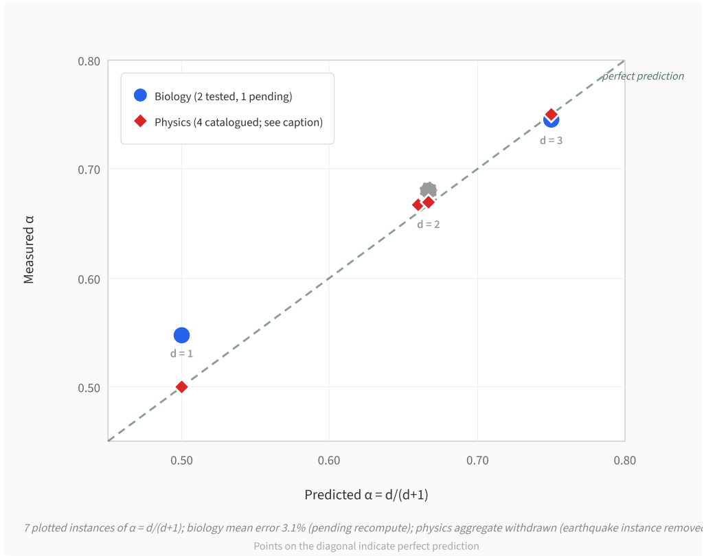
Figure 3 | Predicted vs Measured. Cross-domain instances of one independently derived formula: \alpha = d/(d+1) [17,21,22,23,24,25]. Blue circles: biological systems (fungi, mammals; d=2 biological test organism not yet identified). Red diamonds: physics systems (crystal growth, phase transitions, fracture; earthquake data point removed; retained separately as a variable-pair case study in the text). Points on or near the diagonal indicate accurate prediction. A single equation, with zero adjustable parameters, governs systems spanning biology, geophysics, and condensed matter physics. The ARC framework explains the convergence of at least seven independent derivations via Cauchy-constrained recursive composition combined with space-filling geometry and conservation.
