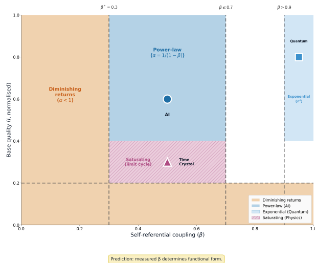
Figure 6. The \beta -Transition Phase Diagram. Scaling regimes as a function of base quality ( I ) and self-referential coupling ( \beta ). AI systems (power-law, \beta \approx 0.5 ), quantum error correction (exponential, \beta > 0.9 ), and time crystals (saturating). Prediction: measured \beta determines functional form.
