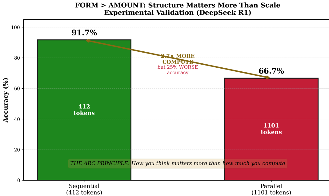
Figure 2 | Sequential recursion compounds: each step builds on prior output ( \alpha > 0 ). Parallel recursion samples independently ( \alpha \approx 0 ). Form of recursion determines the regime. Confirmed across all 5 tested models: sequential \geq parallel in every case.
