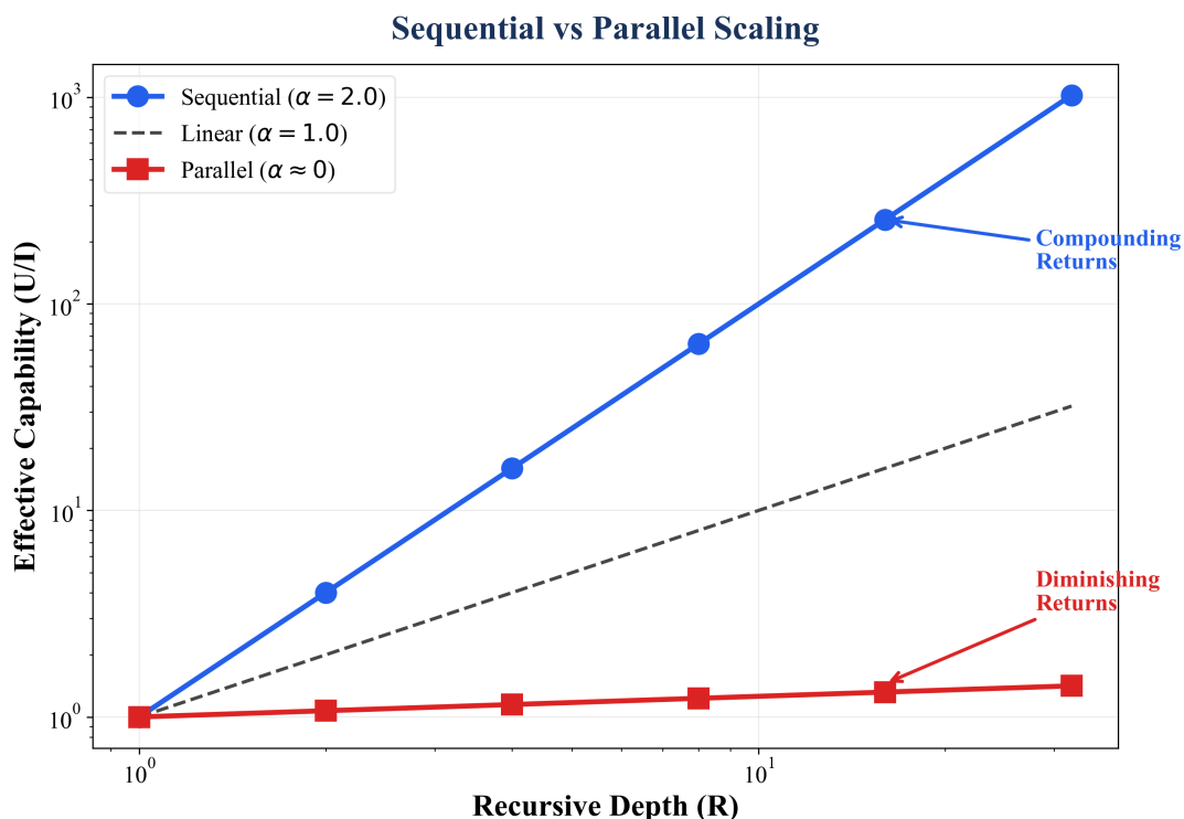
Figure 3 | Scaling Comparison. Log-log plot showing different scaling regimes. Power law U = R^\alpha appears as a straight line with slope \alpha . Sequential recursion ( \alpha > 1 ) illustrates super-linear growth schematically; parallel sampling ( \alpha < 1 ) shows diminishing returns. The ARC Principle originally predicted \alpha_{\text{sequential}} > 1 > \alpha_{\text{parallel}} ; Paper II's multi-model replication (March 2026, see §3.9) confirms \alpha_{\text{parallel}} \approx 0 universally, while the best cross-architecture fit for \alpha_{\text{sequential}} is sub-linear ( \approx 0.49 , Gemini 3 Flash). The directional prediction (sequential > parallel) holds robustly across all six frontier models; the quantitative \alpha > 1 claim is not confirmed cross-architecturally for current frontier systems.
